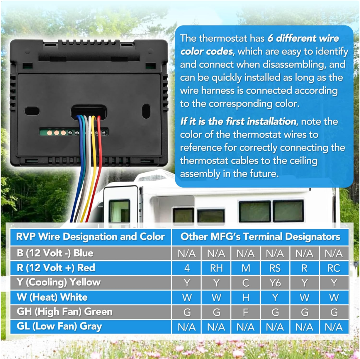
Figure 2.1: Key features of the RV Thermostat, emphasizing its dual heating/cooling capability, user-friendly controls, and simple installation process.
