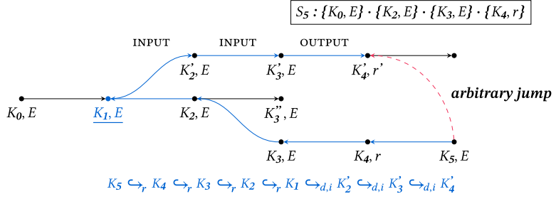
Figure 5-10. Schematic of how the multiverse debugger can jump to any arbitrary state in the past, using the step-back and step-mock rules. For the arbitrary jump from state K_5 to K_4' , the join K_1 is underlined and shown in blue. Top right: the list of snapshots before the arbitrary jump. Bottom: the execution path from K_5 to K_4' . Steps with the step-back and step-back-compensate rules are shown as \xrightarrow{r} .
