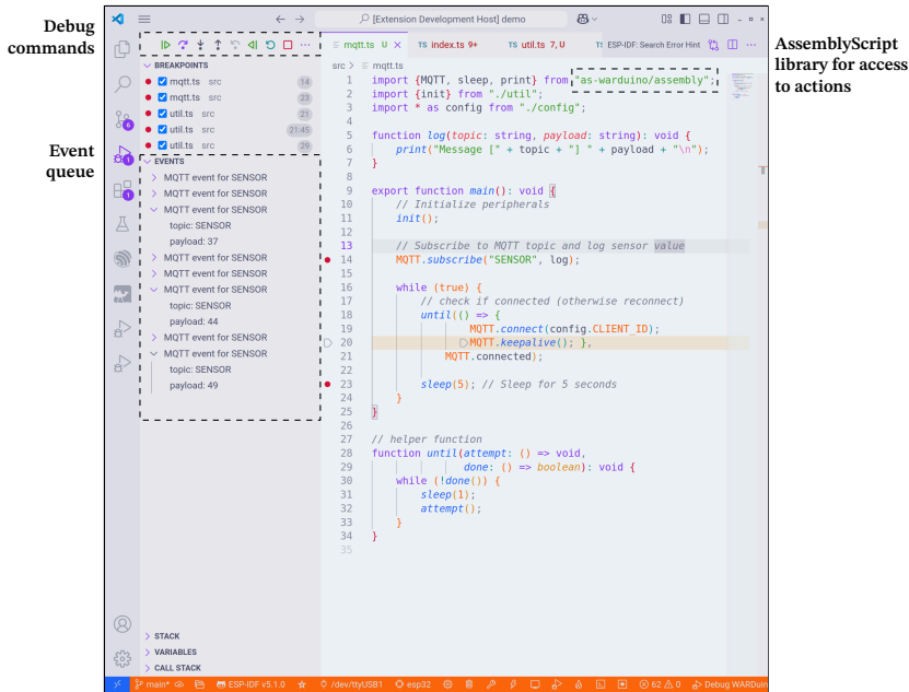
Figure 4-12. A screenshot of the out-of-place debugger in VS Code.
