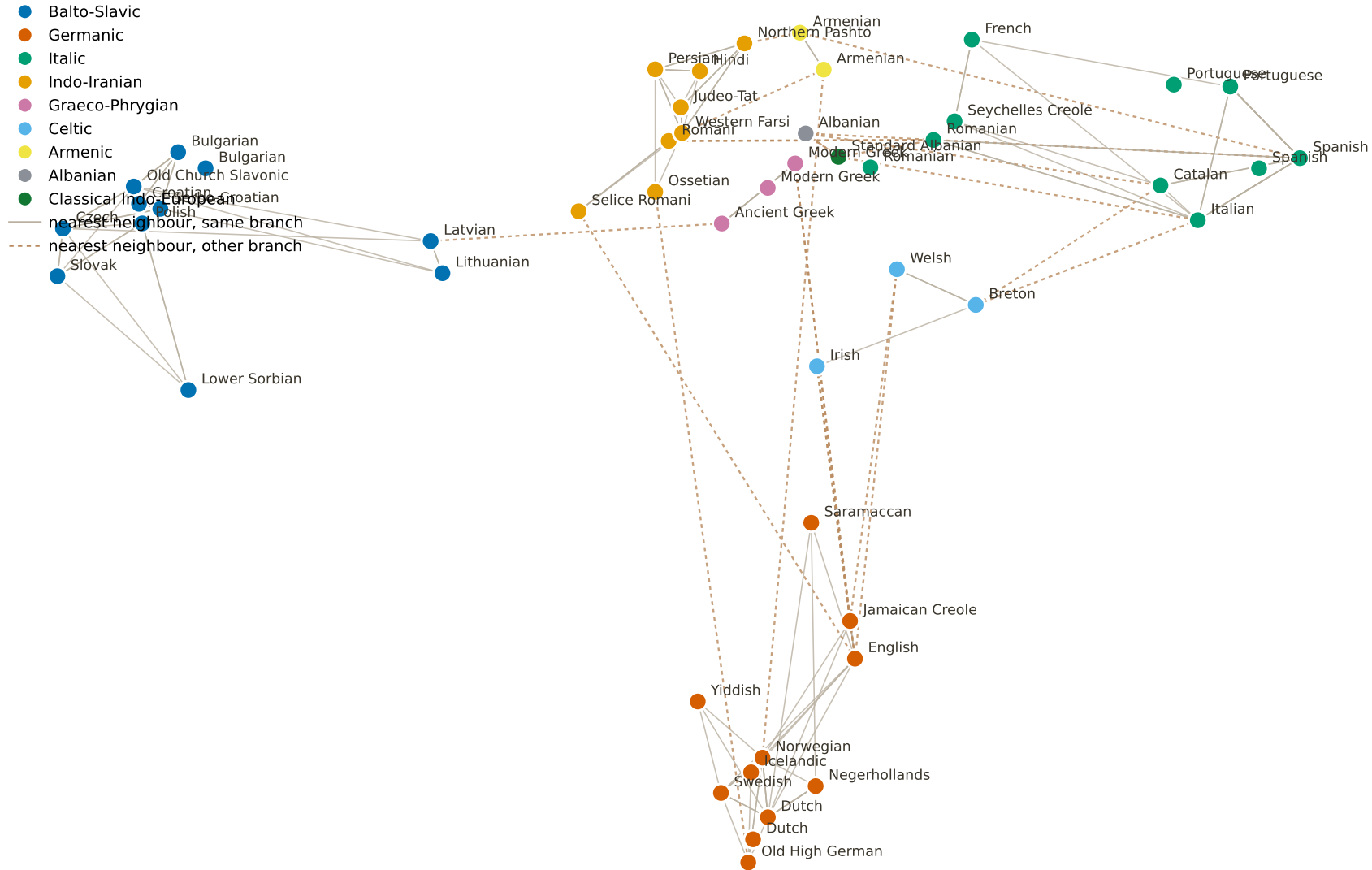
ie50 placed by consonantal-correspondence dissimilarity (MDS)
