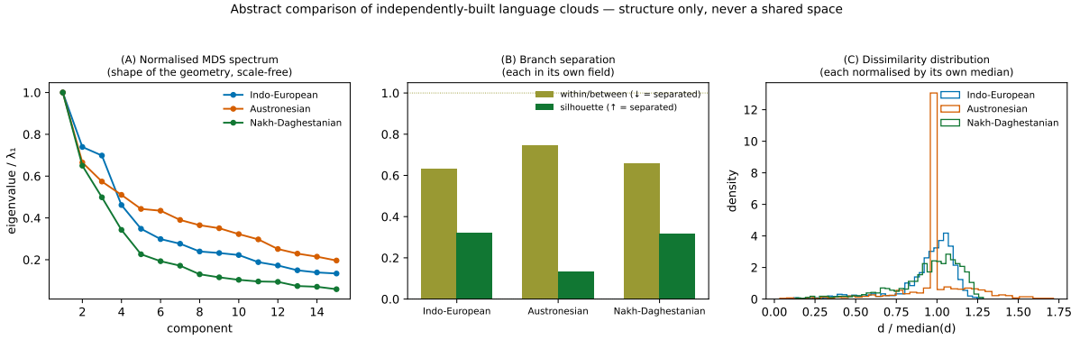
Figure 2: Abstract comparison of the three independently-built clouds — structure only, never a shared space. (A) normalised MDS spectra; (B) branch separation; (C) each cloud’s dissimilarity distribution normalised by its own median.
