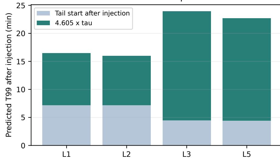
D. Forecast decomposition
