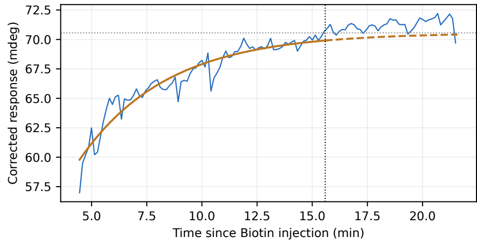
L5: channel 2, 785 nm; \tau = 3.96 min
