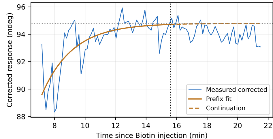
L3: channel 2, 670 nm; \tau = 4.23 min
