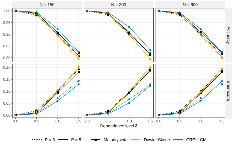
Fig. 2 Classification accuracy (top) and Brier score (bottom) of the posterior class probabilities by dependence level \delta ; layout as in Fig. 1
