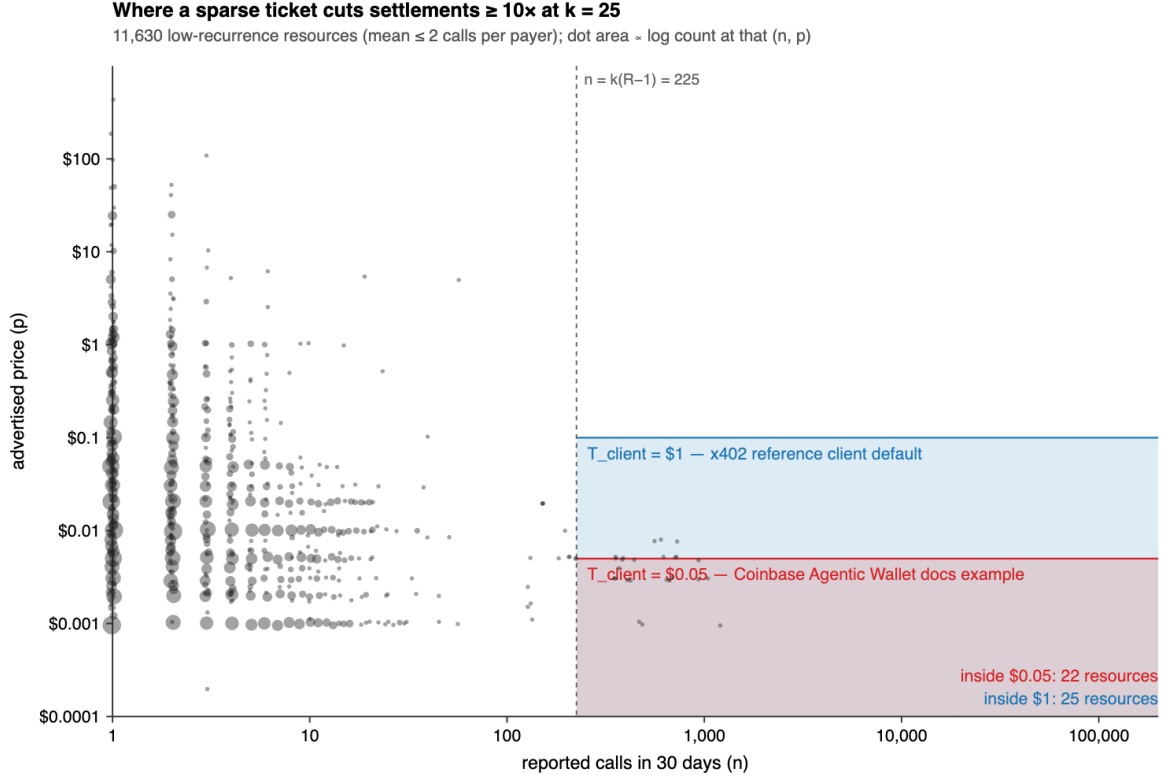
Figure 1: Every low-recurrence resource in the index against the two boundaries the measured client caps imply. The vertical line is the merchant-variance bound n \geq k(R - 1) ; the horizontal lines are the client caps.
