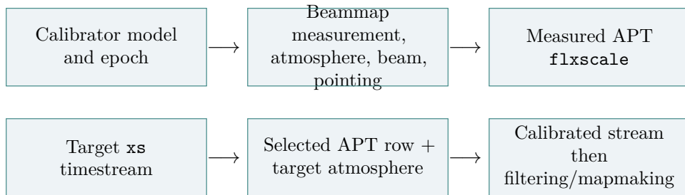
Figure 1: Scientific lineage from calibrator evidence to target-observation calibration. TolProj selects or produces the observation-specific APT; SCI-CAL consumes its selected flxscale and applies target atmosphere once.
