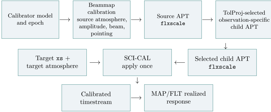
Figure 1: Scientific lineage from calibrator evidence to target-observation calibration. Beammap calibration produces the source APT factor; TolProj selects or creates the observation-specific child APT; SCI-CAL consumes its selected flxscale and applies the target atmosphere once.
