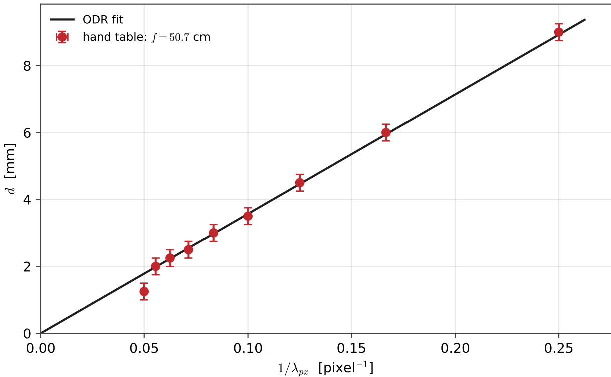
SLM focal-length fit: new f = 50.7 \pm 1.5 cm ( \chi^2/\nu = 0.61 )
