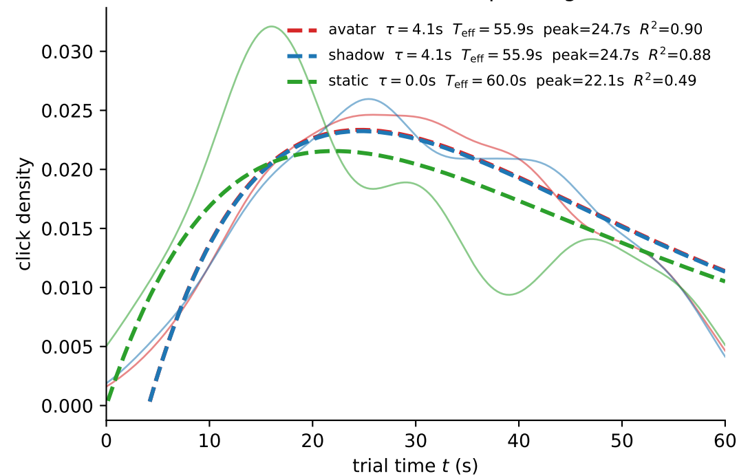
B S(t) = A \cdot u \cdot e^{-\lambda u} fits per target
