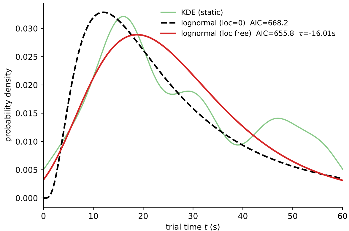
lognormal family — lag vs no-lag
