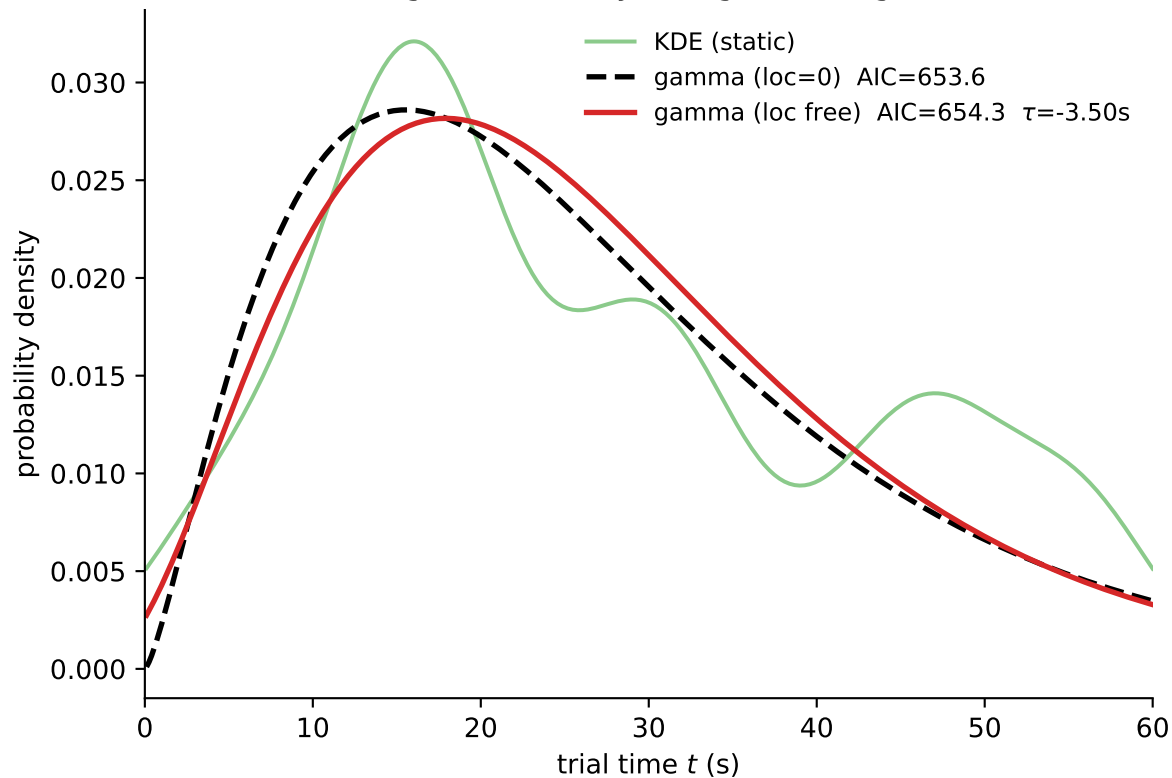
gamma family — lag vs no-lag
