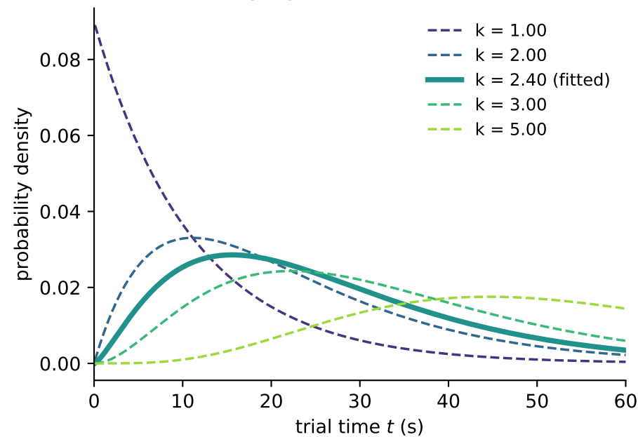
A varying k at fixed \theta = 11.13 s
