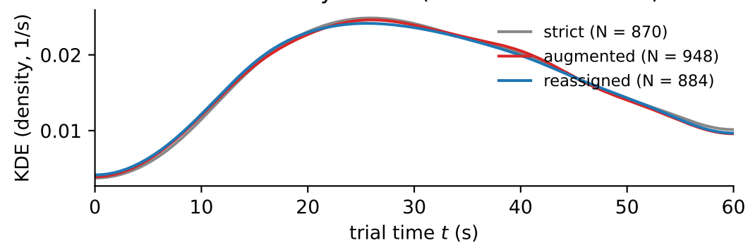
Matlab KDE by cohort (reflection-corrected)
