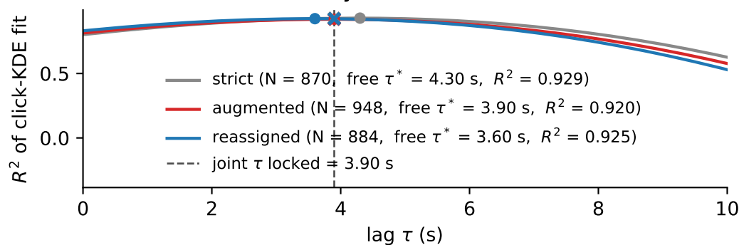
Cohort sensitivity (locked \tau marked with \times )
