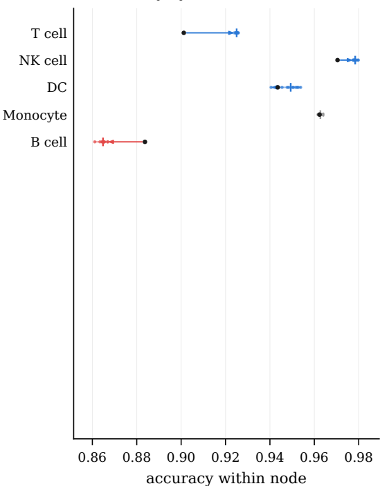
L2 accuracy by true L1
