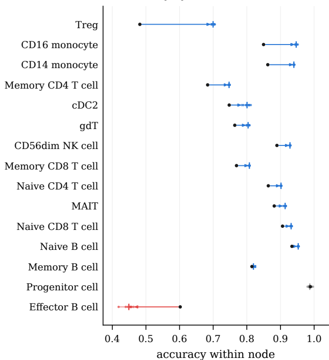
L3 accuracy by true L2
