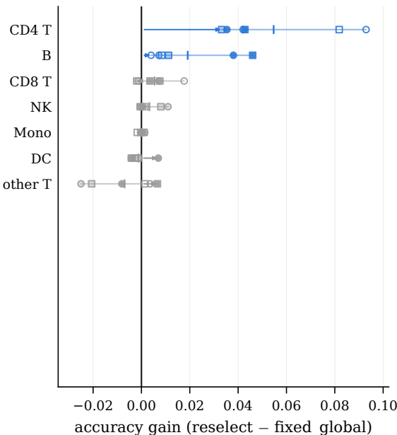
L2 gain by true L1
