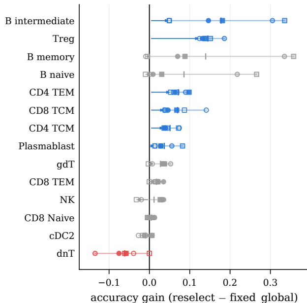
L3 gain by true L2
