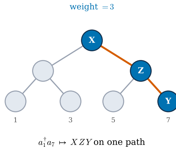
(b) tree encoding: balanced tree
