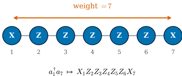
(a) Jordan-Wigner: linear chain
