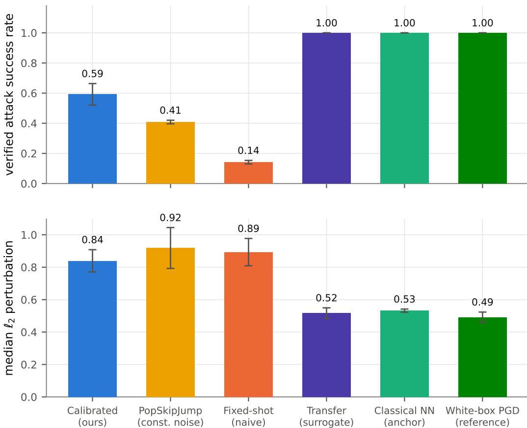
RQ1 Hard-label attacks on a variational quantum classifier (success is verified against the exact model; bars are mean \pm s.d. over seeds)
