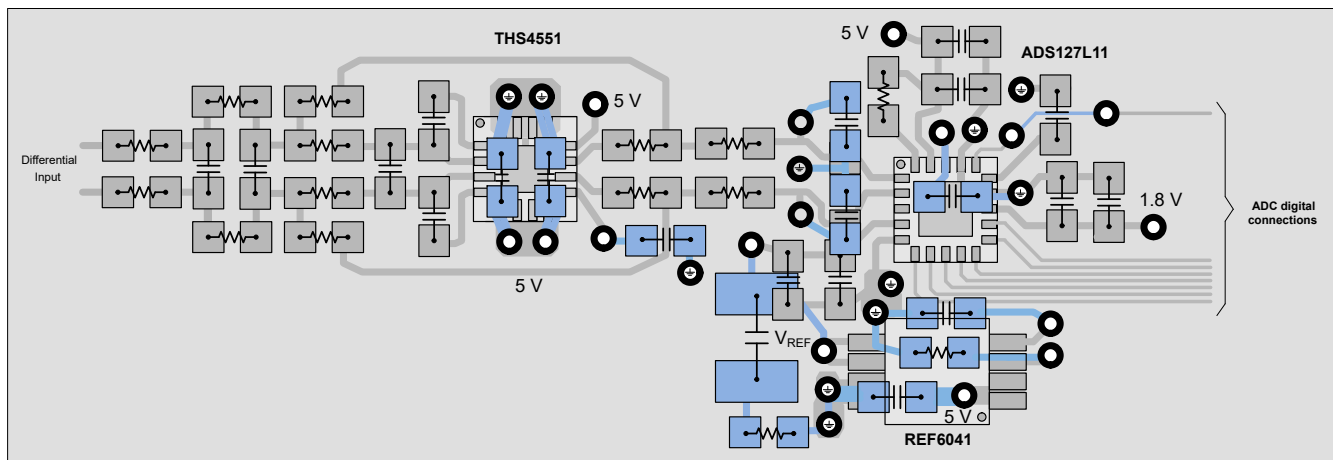
Figure 11-1. Layout Example of Typical Application Circuit
