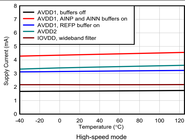
Figure 6-59. Power-Supply Current vs Temperature
