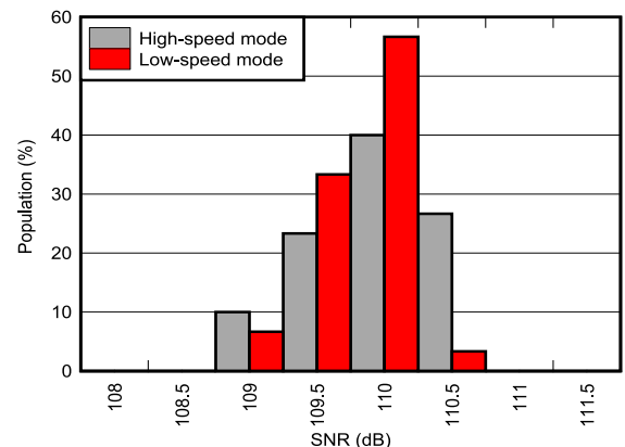
Figure 6-25. SNR Distributions
