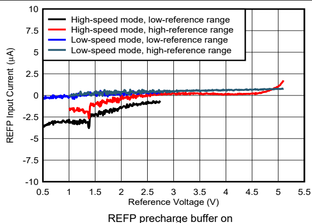
Figure 6-55. REFP Input Current vs Reference Voltage
