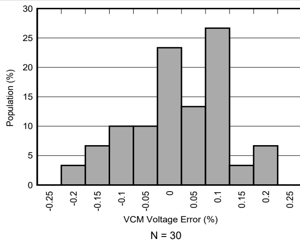
Figure 6-52. VCM Voltage Distribution
