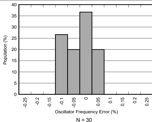
Figure 6-50. Oscillator Frequency Distribution
