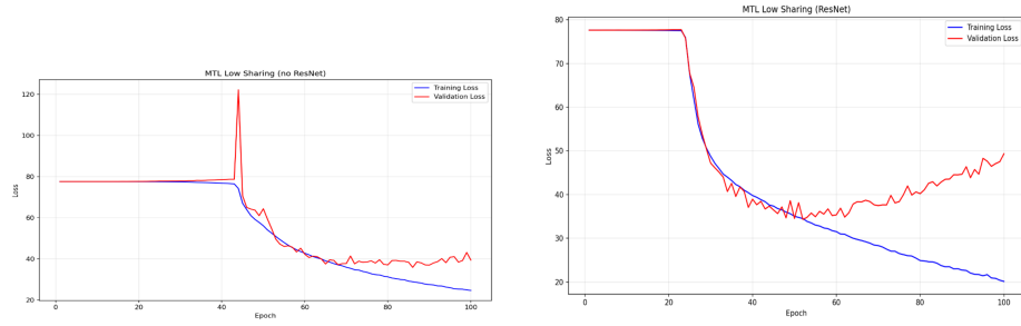
(a) CNN backbone: plateau lasts \approx 40 epochs before a sharp transition, with a large validation spike around epoch 44. (b) ResNet backbone: plateau breaks at \approx 22 epochs and convergence is monotonic; validation diverges only past epoch 50.
