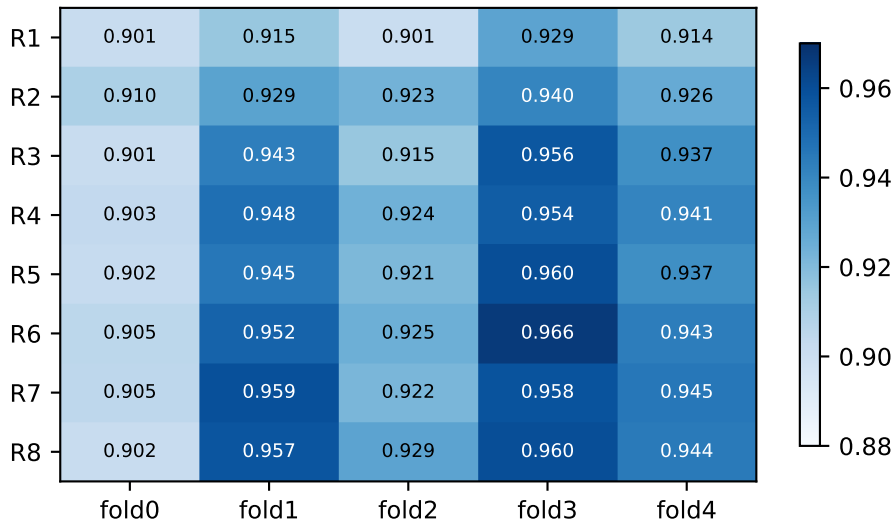
EfficientNet-B0 (all rounds × folds)
