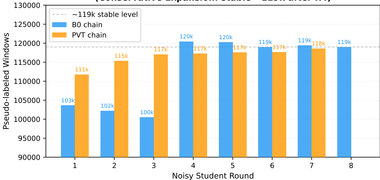
Pseudo-Label Count Per Round (Conservative Expansion: stable ~119k after R4)
