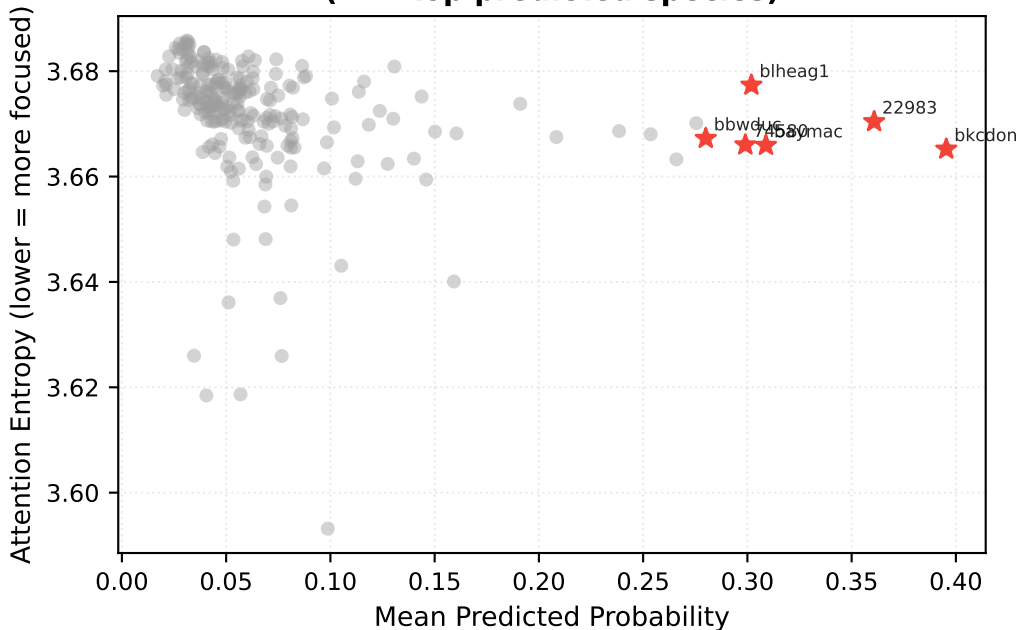
B0 R8: Probability vs Attention Focus (★ = top predicted species)
