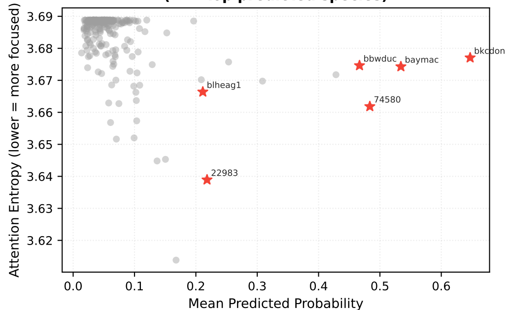
PVT R8: Probability vs Attention Focus (★ = top predicted species)
