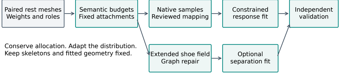
Figure 1: SBCST separates invariant influence allocation from task-dependent fitting. The upper branch preserves authored response under new body proportions. The lower branch addresses footwear whose fitted extent makes target-body spatial association a more useful objective. Both branches retain clothing dynamics and use independent validation before writeback.
