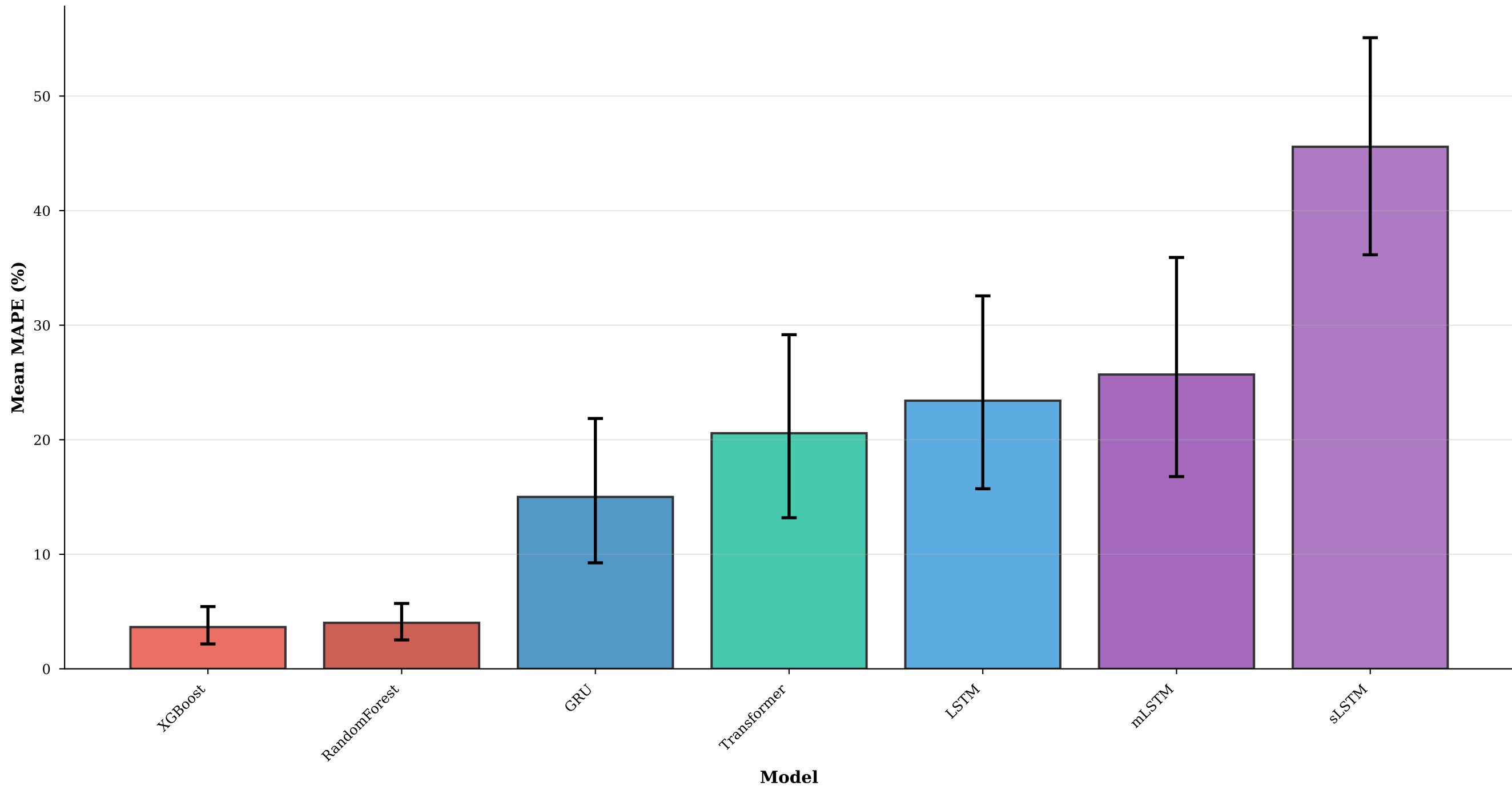
Model Performance with 95% Bootstrap Confidence Intervals (Averaged Across All Indicators)
