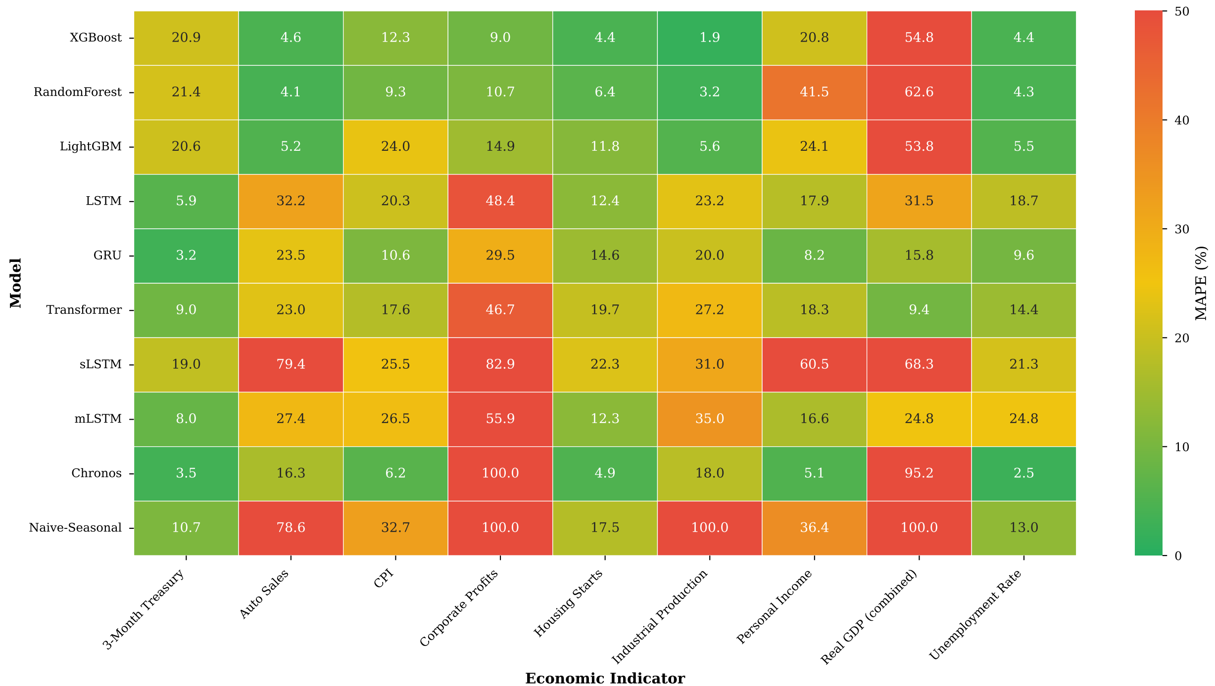
Forecast Accuracy Heatmap: MAPE (%) Across Models and Indicators (Lower is Better)
