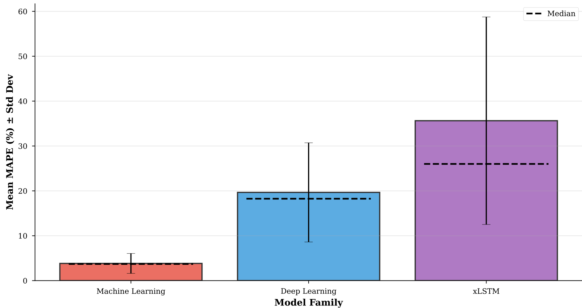
Model Family Performance Comparison (Error bars show standard deviation, dashed line shows median)
