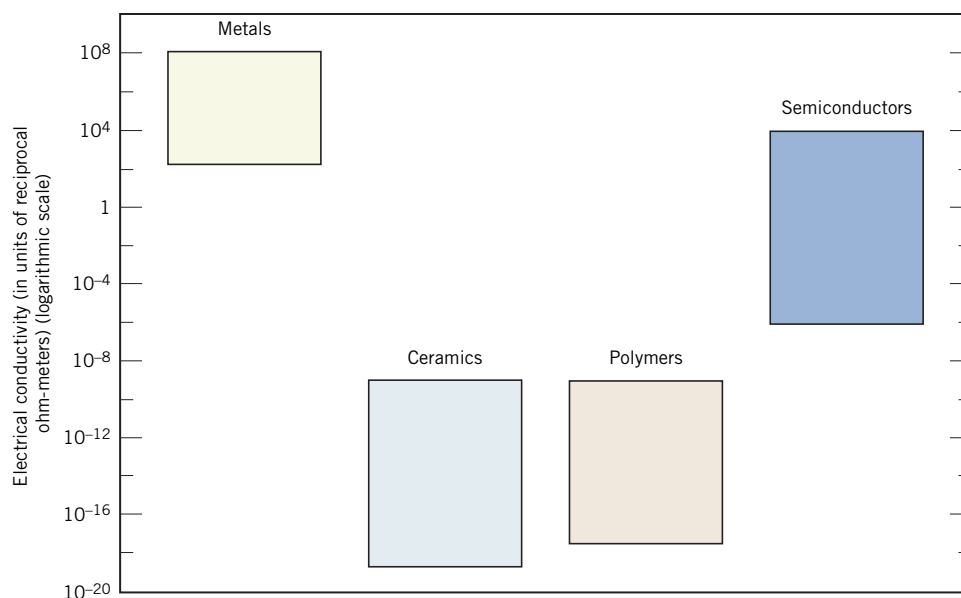
Figure 1.8 Bar chart of room-temperature electrical conductivity ranges for metals, ceramics, polymers, and semiconducting materials.
