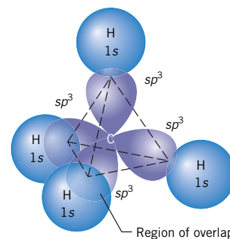
Figure 2.15 Schematic diagram that shows bonding of carbon sp^3 hybrid orbitals to the 1s orbitals of four hydrogen atoms in a molecule of methane ( CH_4 ). (From J. E. Brady and F. Senese, Chemistry: Matter and Its Changes , 4th edition. Reprinted with permission of John Wiley & Sons, Inc.)
