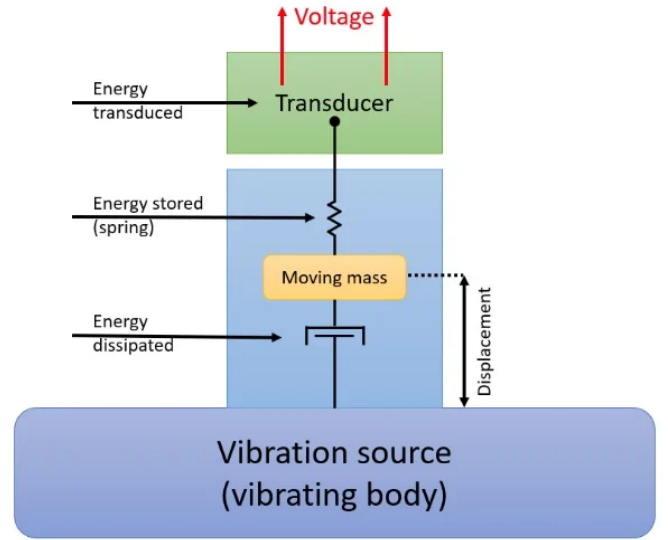
Fig. 2. Vibrational energy harvesting principle ?
