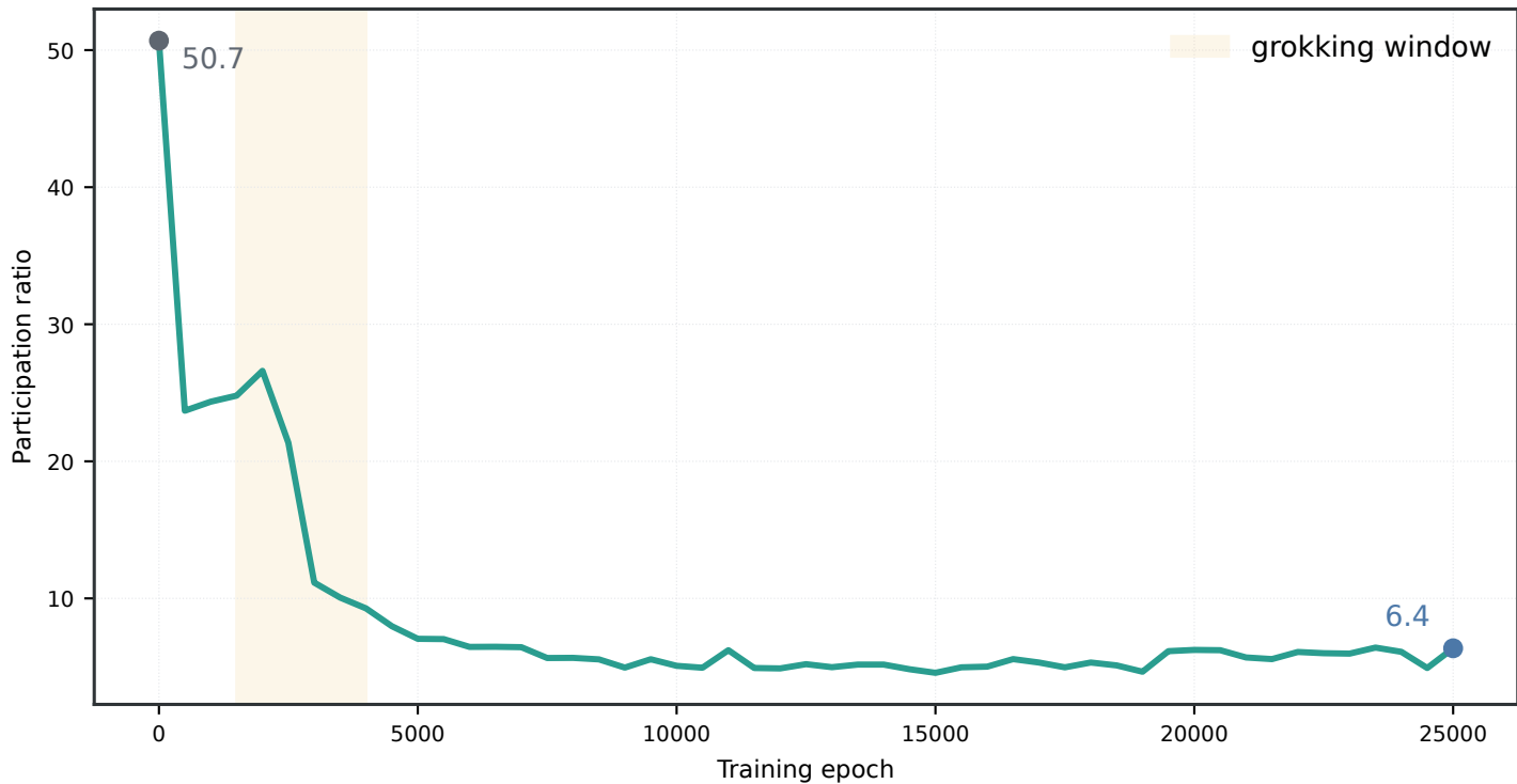
Hidden activations collapse to a low-dimensional representation
