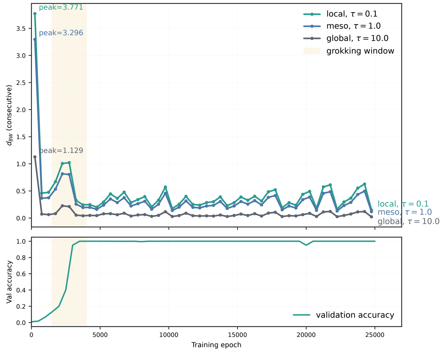
Heat-kernel BW distances across diffusion scales
