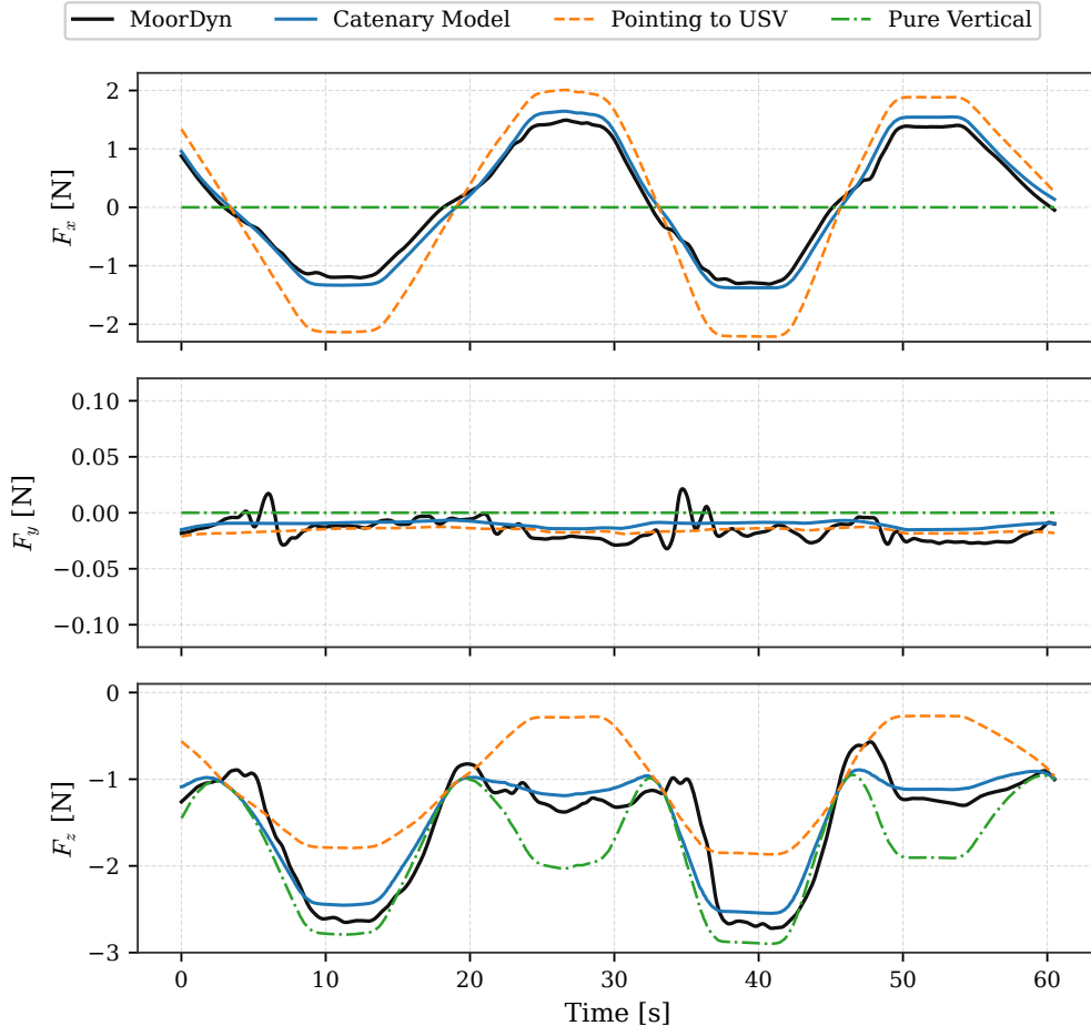
Figure 4.15: Three-dimensional tether force components at the UAV.
