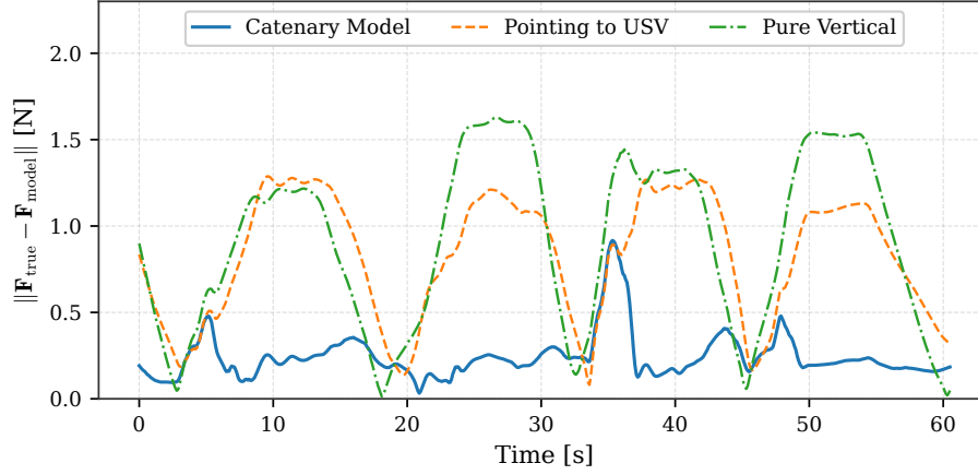
Figure 4.16: Three-dimensional tether force error norm.
