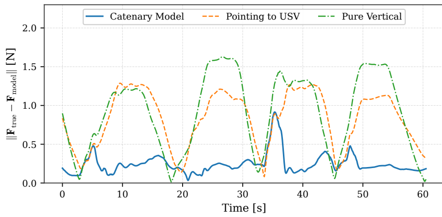
Figure 4.13: Three-dimensional tether force error norm.
