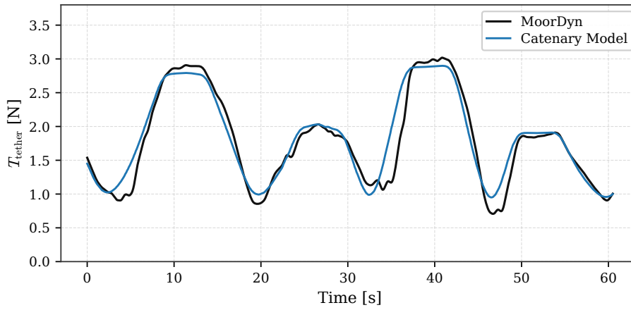
Figure 4.11: Tether tension magnitude at the UAV.
