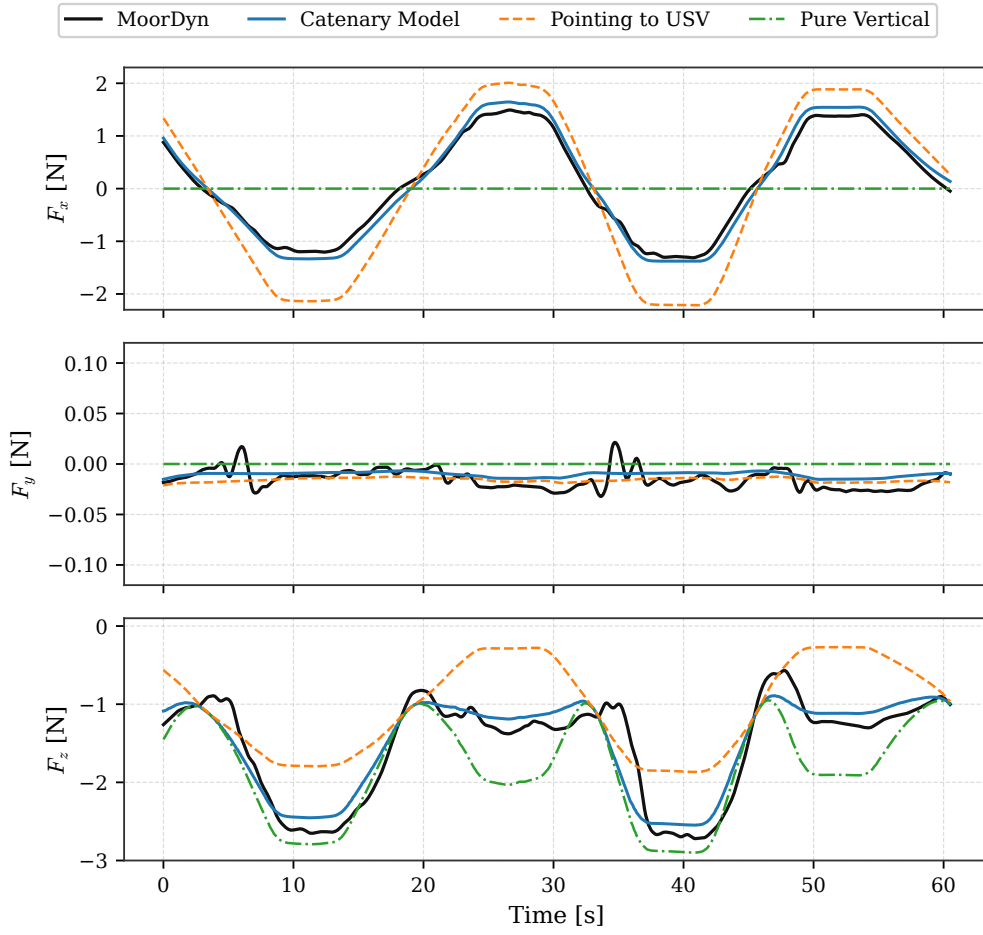
Figure 4.12: Three-dimensional tether force components at the UAV.
