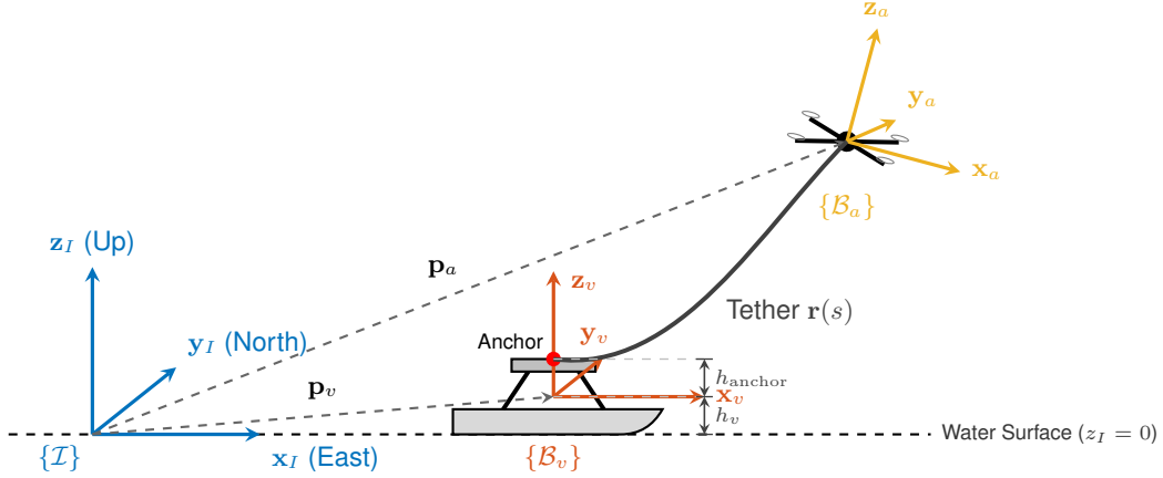
Figure 3.1: Reference coordinate frames \{I\} , \{B_v\} , \{B_a\} , and anchor connection.
