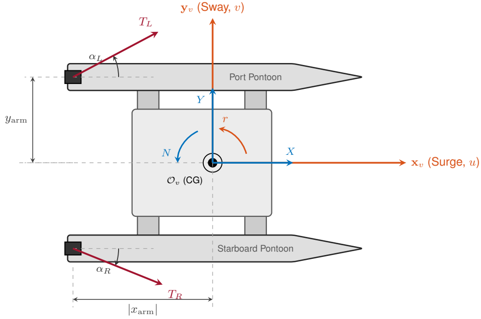
Figure 3.2: Planar 3-DOF USV schematic and thruster allocation geometry.
