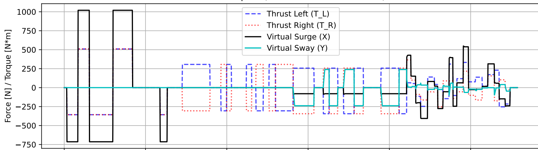
Control Inputs (Thruster &amp; Virtual Forces)
