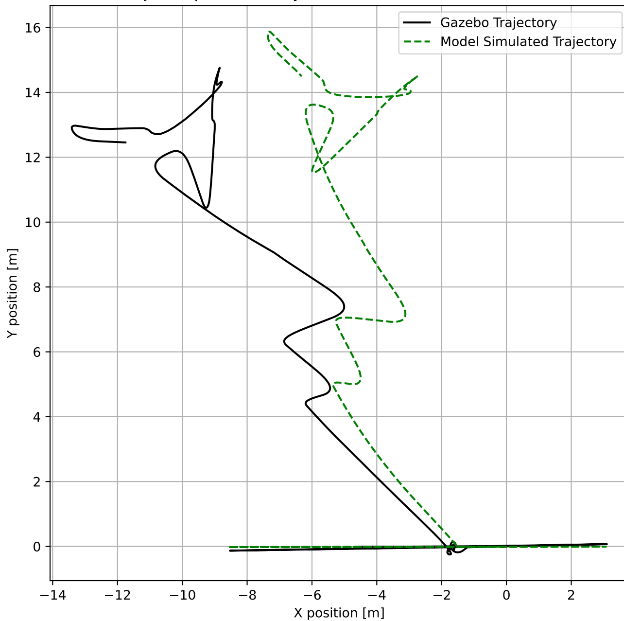
Traj. Comparison (Body-to-Global Kinematics Validation)
