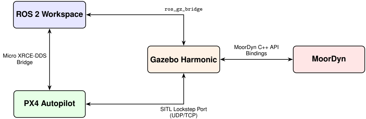
Figure 3.1: Simulation software ecosystem and communication interfaces.
