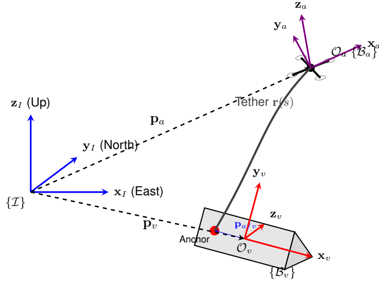
Figure 3.1: Schematic representation of the reference coordinate frames \{I\} , \{B_v\} , \{B_a\} , and the physical anchor connection.
