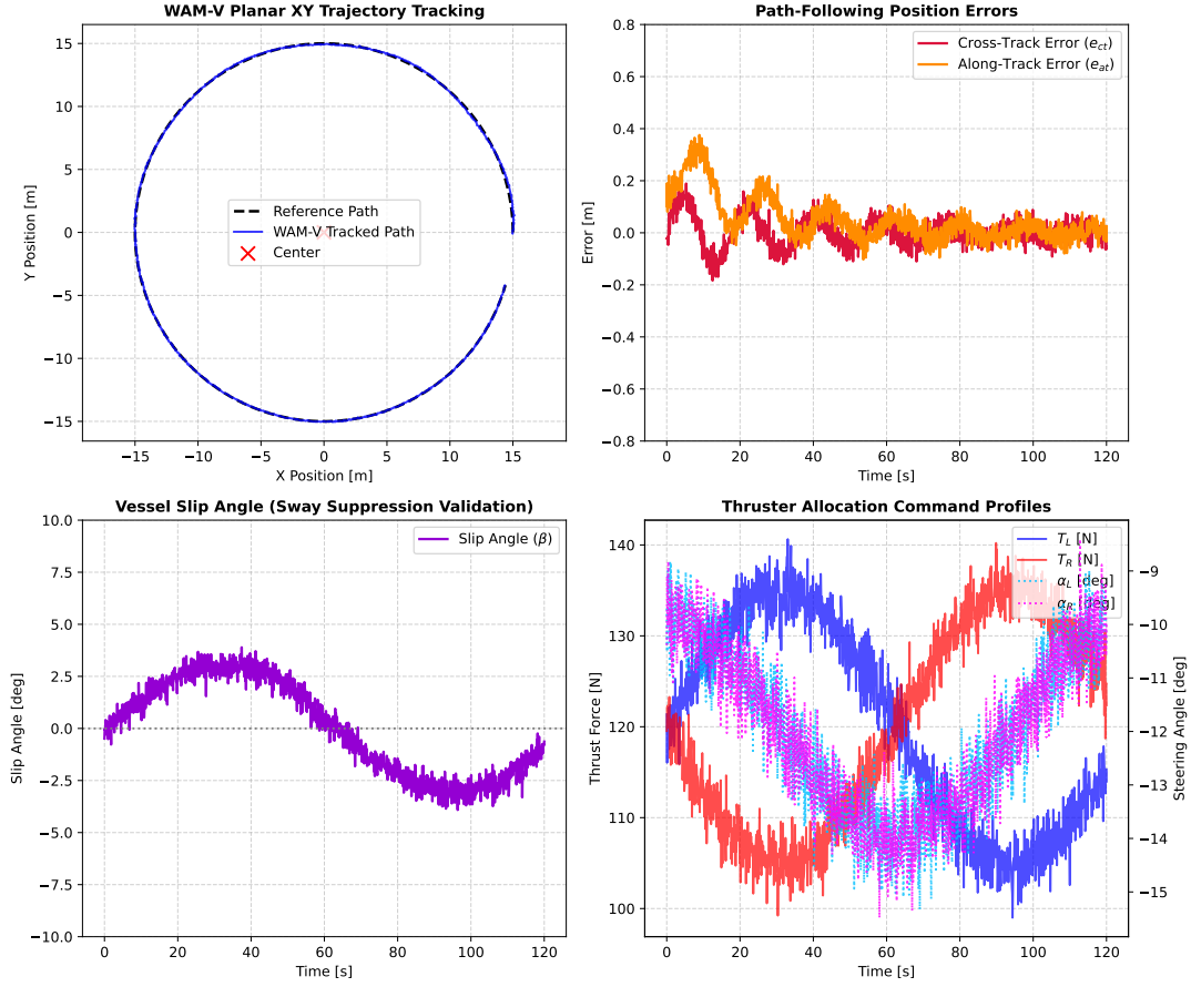
Figure 6.1: WAM-V catamaran planar path-following performance showing the tracked XY path and the corresponding tracking error metrics.
