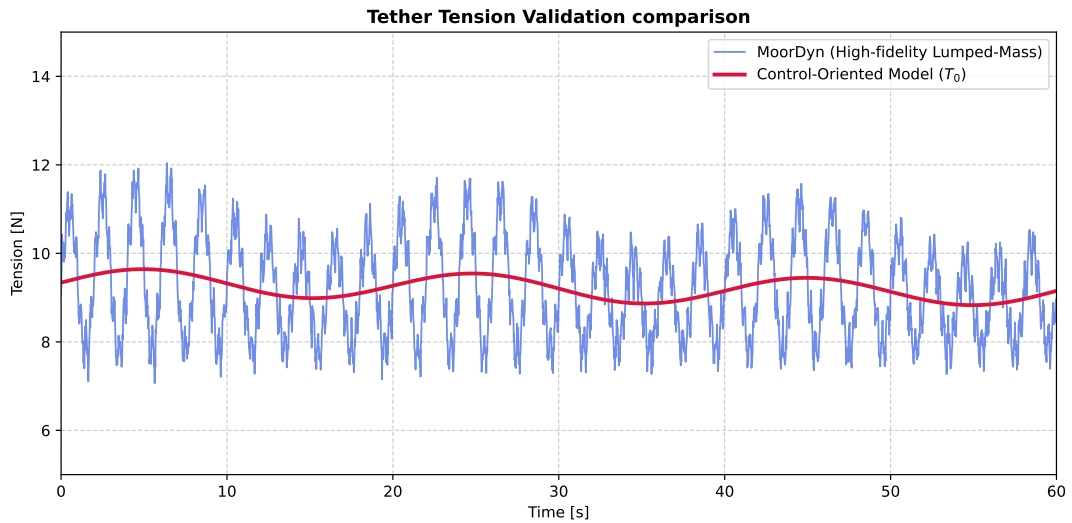
Figure 3.6: Validation of the control-oriented tether tension model ( T_0 ) compared against the high-fidelity MoorDyn multi-node lumped-mass simulation.
