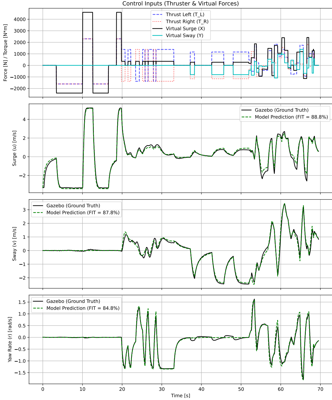
Figure 3.3: Predicted versus ground-truth velocity profiles ( u, v, r ) under the validation excitation sequence.
