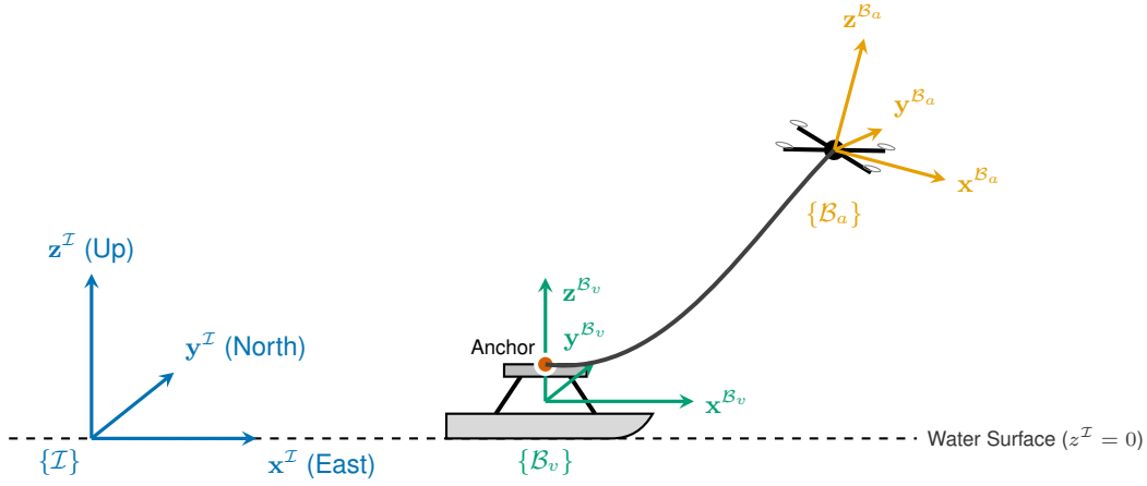
Figure 3.1: Reference coordinate frames \{\mathcal{I}\} , \{\mathcal{B}_v\} , and \{\mathcal{B}_a\} .
