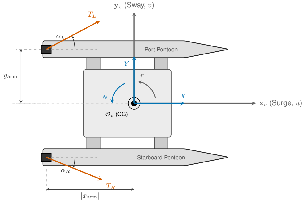
Figure 3.2: Planar USV schematic and thruster allocation geometry.
