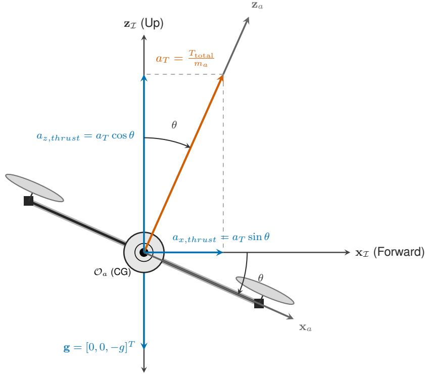
Figure 3.3: Quadrotor thrust vectoring in the longitudinal plane showing body tilt, thrust decomposition, and gravity.
