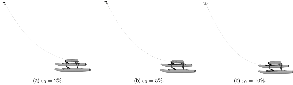
Figure 4.9: Shape of the tether for different slack ratios, displayed in Foxglove.
