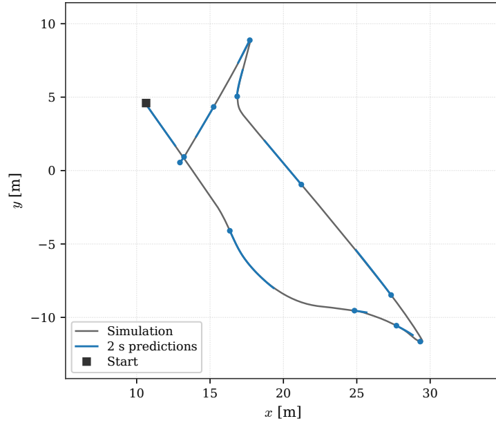
Figure 4.13: USV trajectory validation with two-second receding-horizon predictions overlaid on the simulation ground truth.
