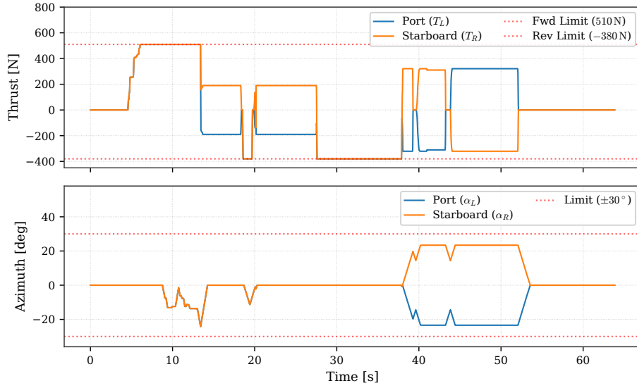
Figure 4.11: USV thruster inputs during the validation maneuver.
