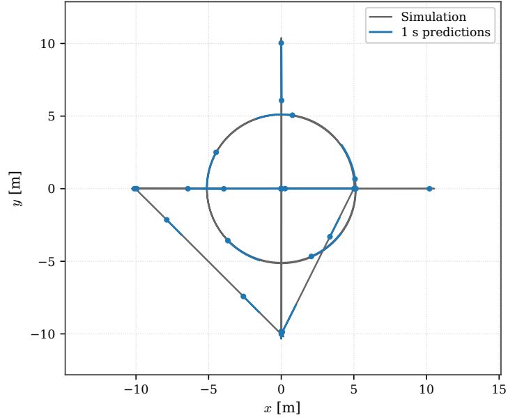
Figure 4.18: One-second open-loop spatial predictions along the flight trajectory.
