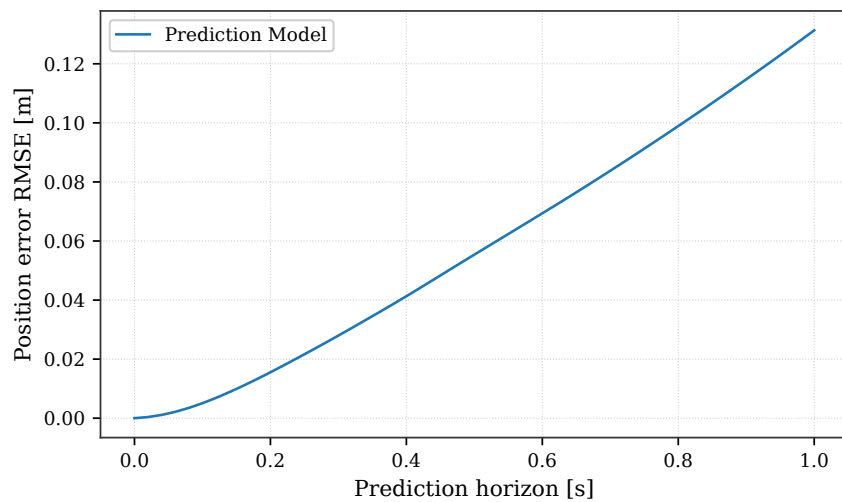
Figure 4.17: UAV position prediction error RMSE as a function of the prediction horizon.
