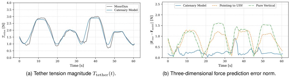
Figure 4.20: Tether tension magnitude and three-dimensional prediction error norm compared against MoorDyn telemetry.
