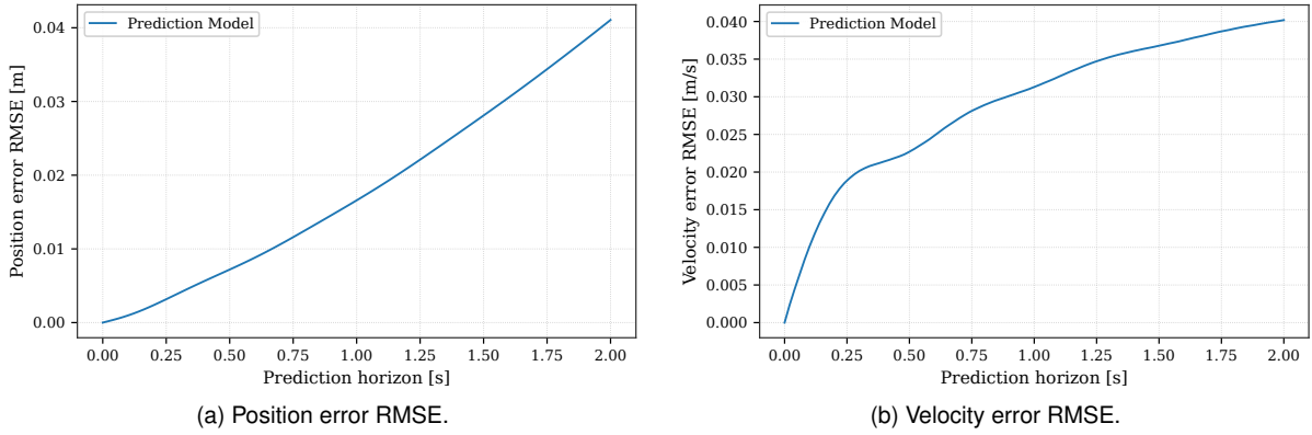
Figure 4.14: USV open-loop prediction error RMSE as a function of the prediction horizon.
