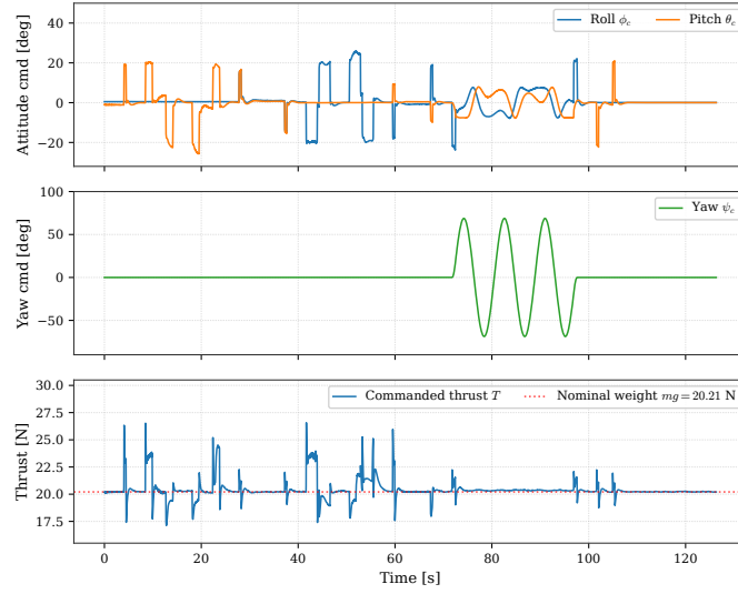
Figure 4.15: UAV attitude and thrust commands during the validation flight.
