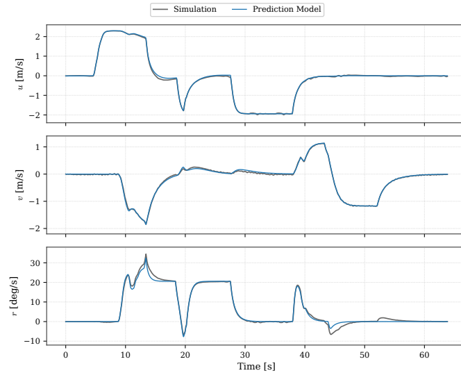
Figure 4.12: USV body-fixed velocities validation.
