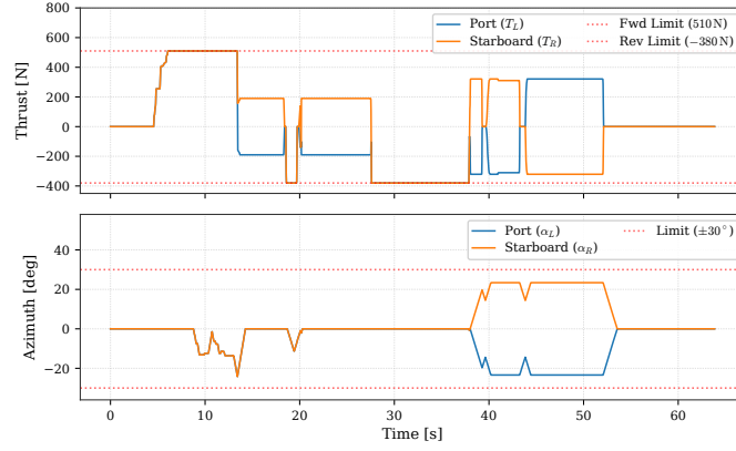
Figure 4.11: USV thruster inputs during the validation maneuver.
