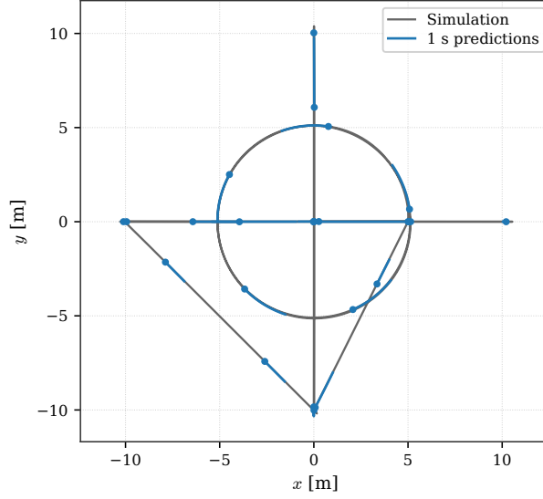
Figure 4.19: One-second open-loop predictions along the UAV flight trajectory.
