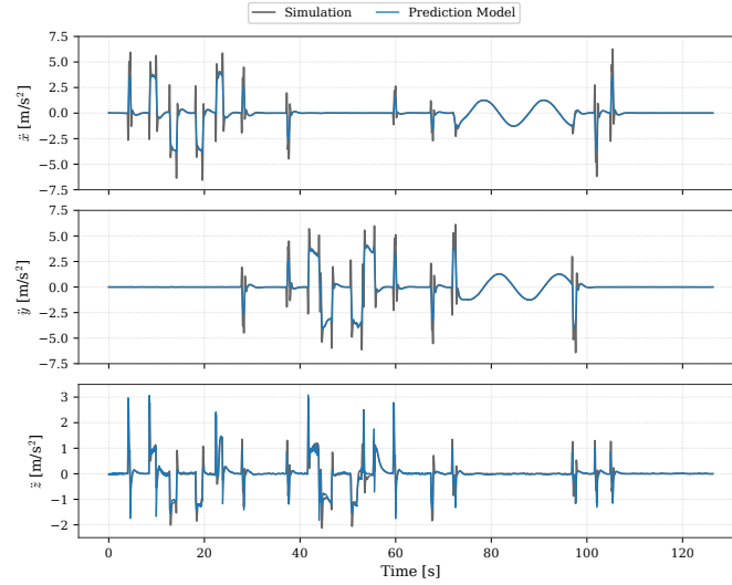
Figure 4.17: UAV inertial acceleration. Ground truth and model driven by the measured attitude.
