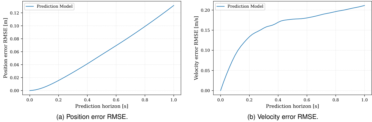
Figure 4.18: UAV open-loop prediction error RMSE as a function of the prediction horizon.
