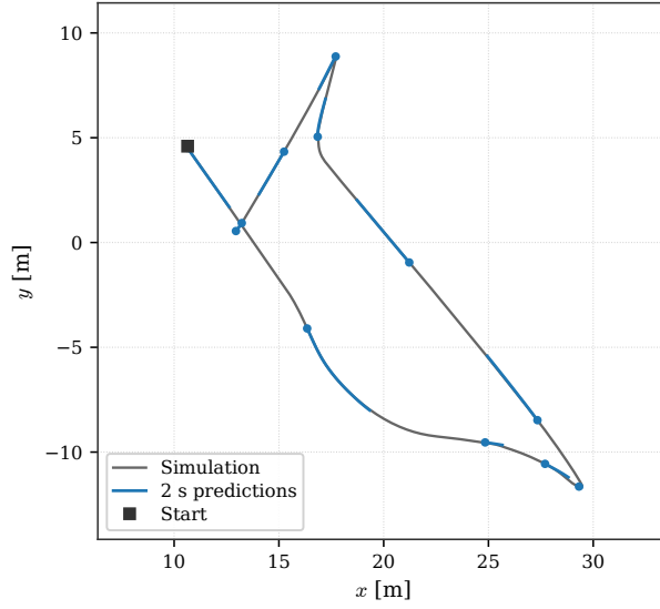
Figure 4.13: Two-second open-loop predictions along the USV trajectory.
