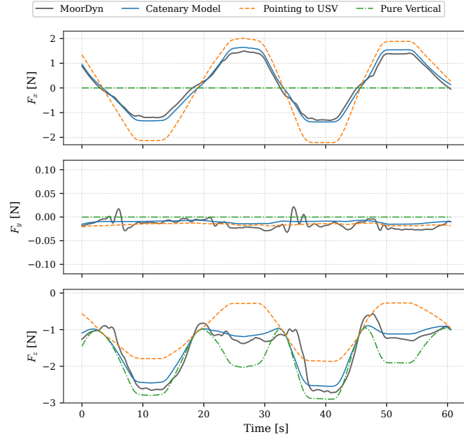
Figure 4.21: Three-dimensional tether force components at the UAV.
