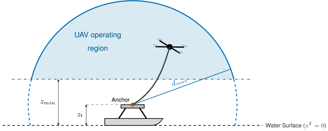
Figure 4.2: Operating region of the UAV.
