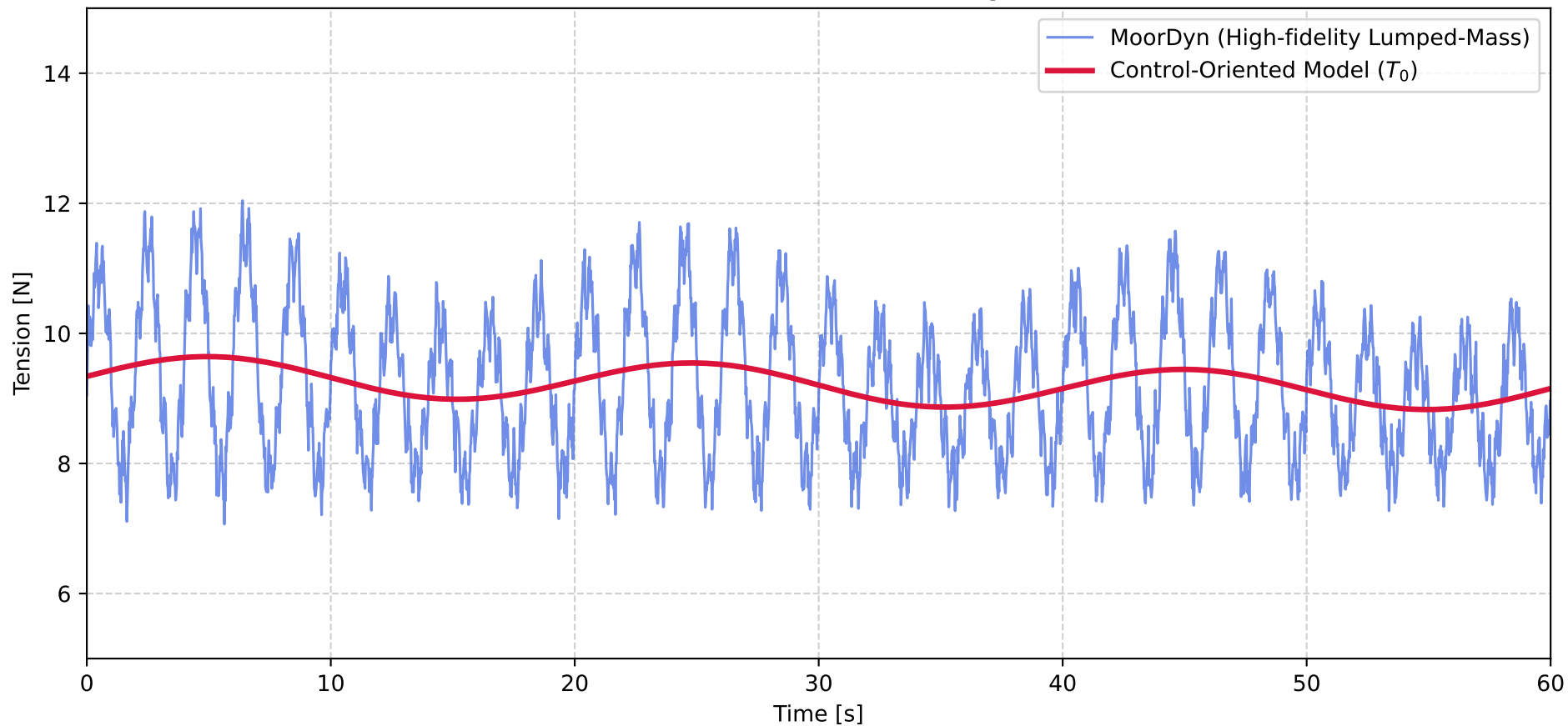
Tether Tension Validation comparison
