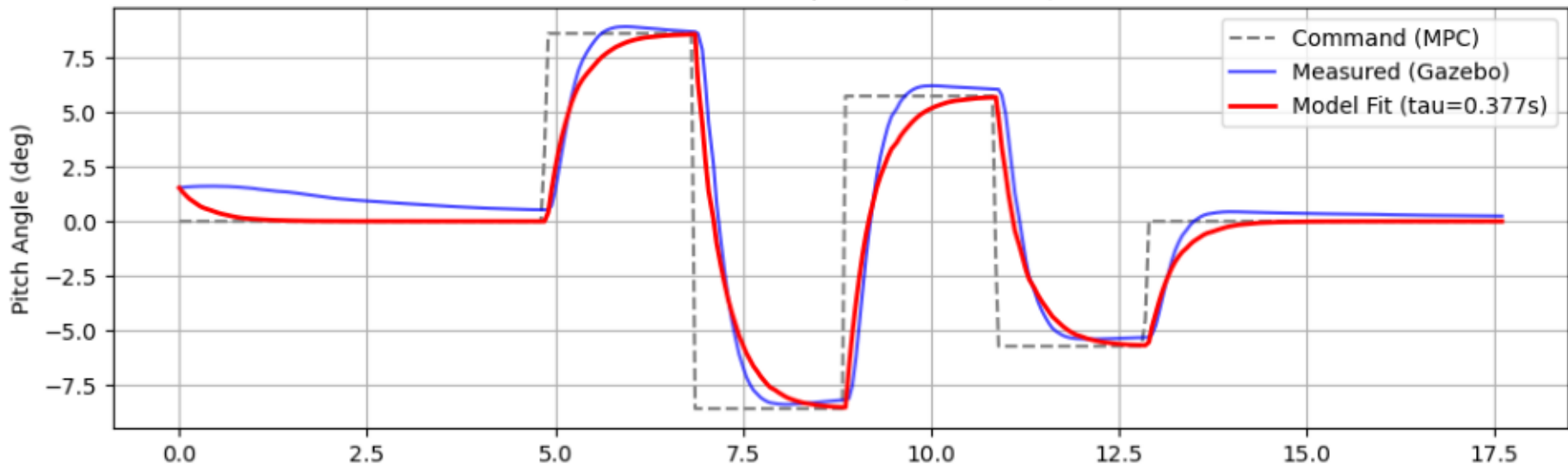
Vertical Dynamics Response ( R^2=-1063.1\% )
