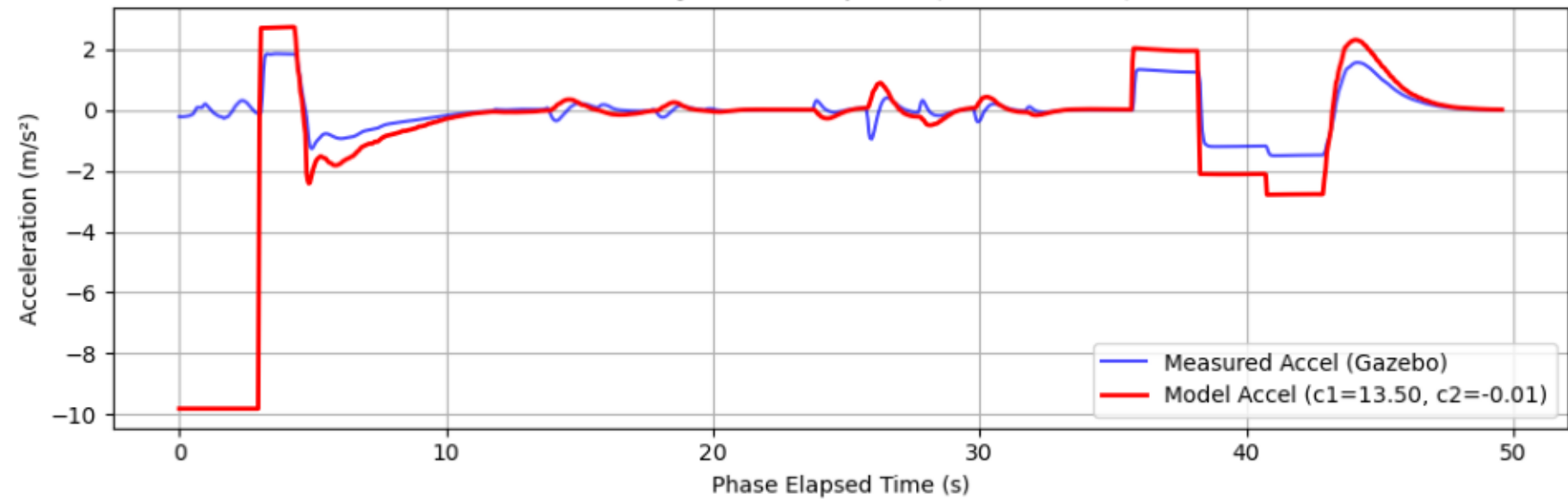
Vertical Dynamics Response ( R^2=-1063.1\% )
