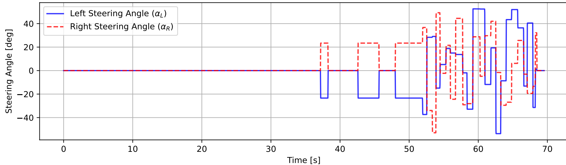
WAM-V Excitation Signals - Steering Angles
