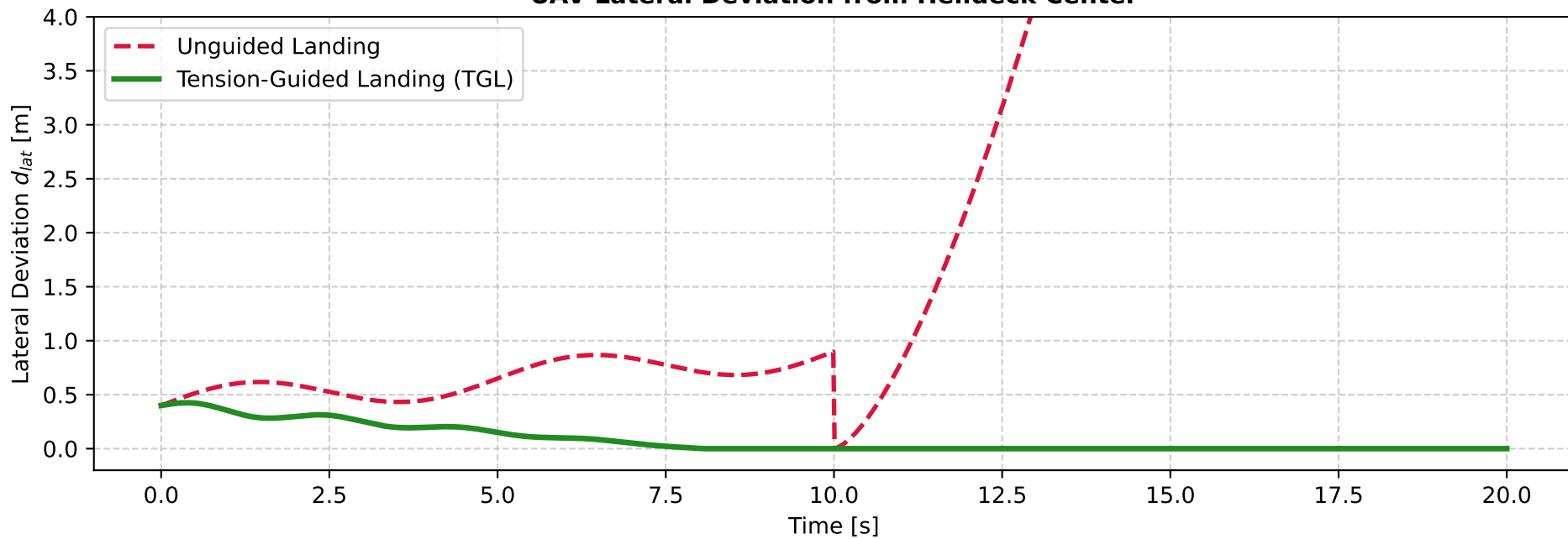
UAV Lateral Deviation from Helideck Center
