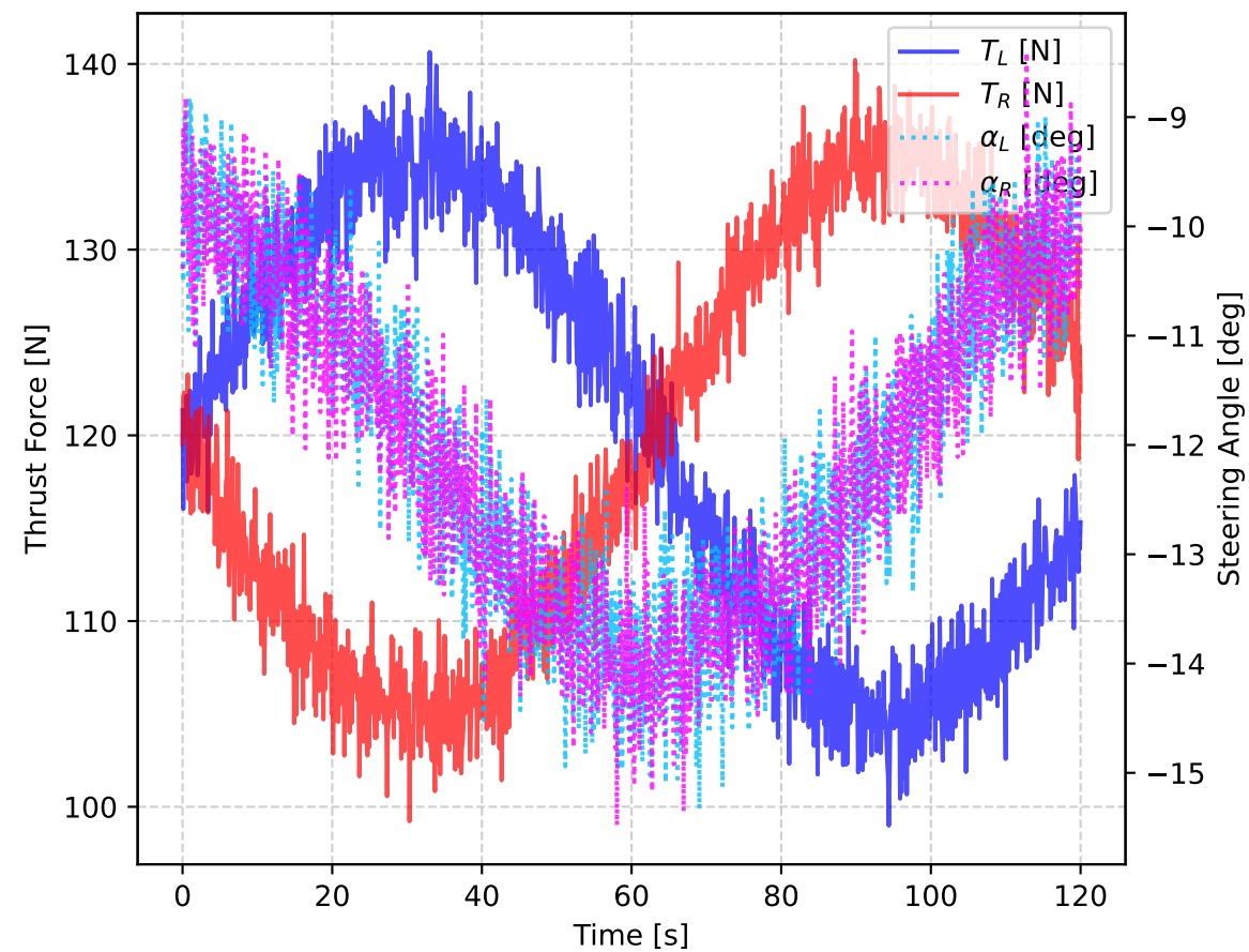
Thruster Allocation Command Profiles
