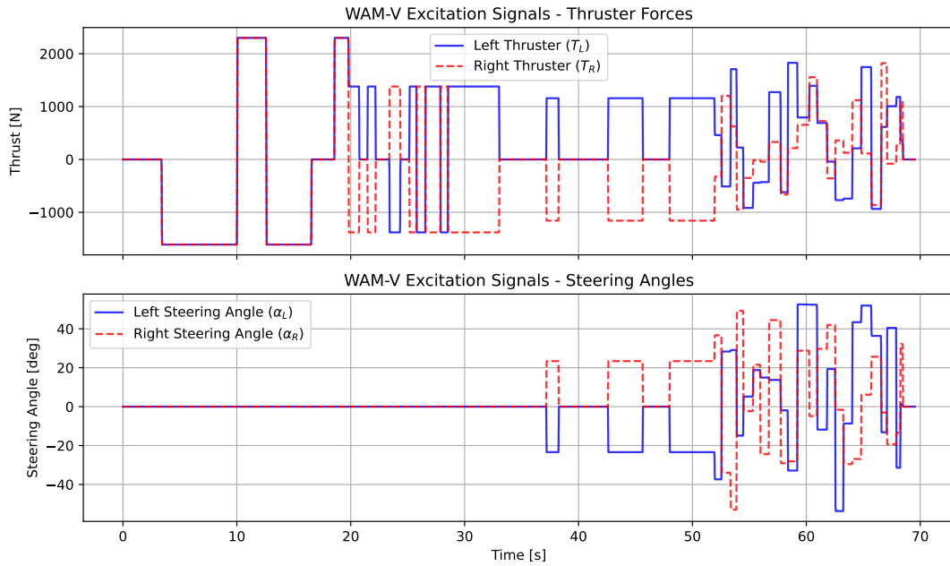
Figure 4.2: Multi-phased excitation signals command profiles (forces and angles) for the WAM-V parameter validation.
