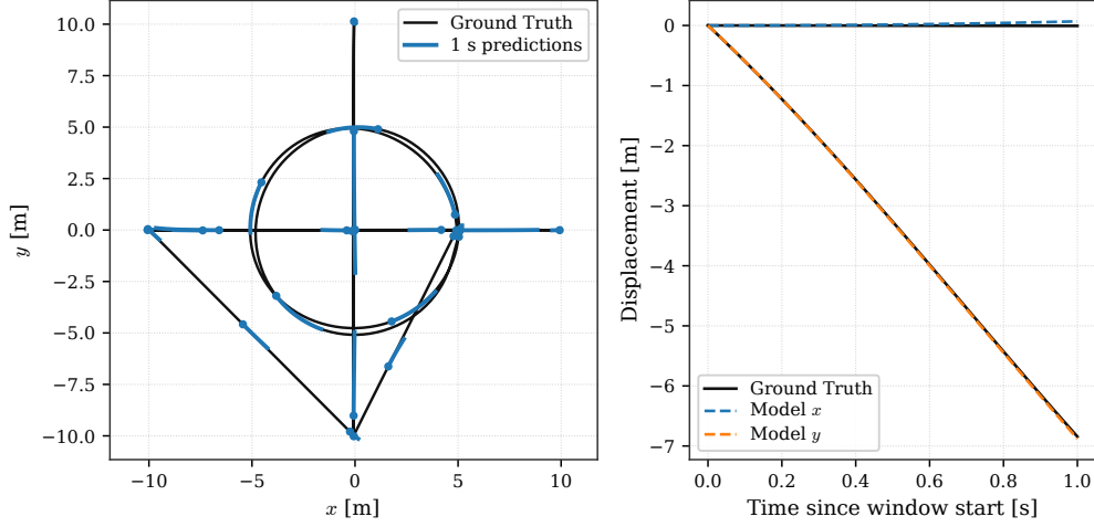
Figure 4.18: One-second open-loop predictions along the flight, and detail of the window with the highest speed.
