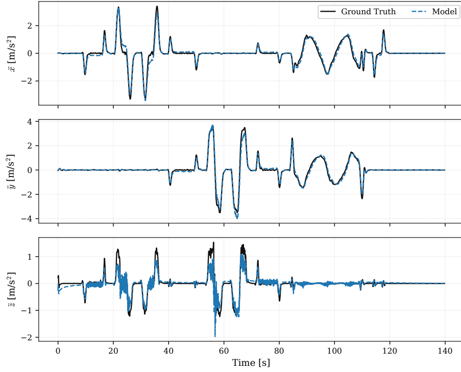
Figure 4.16: UAV inertial acceleration. Ground truth and model driven by the measured attitude.
