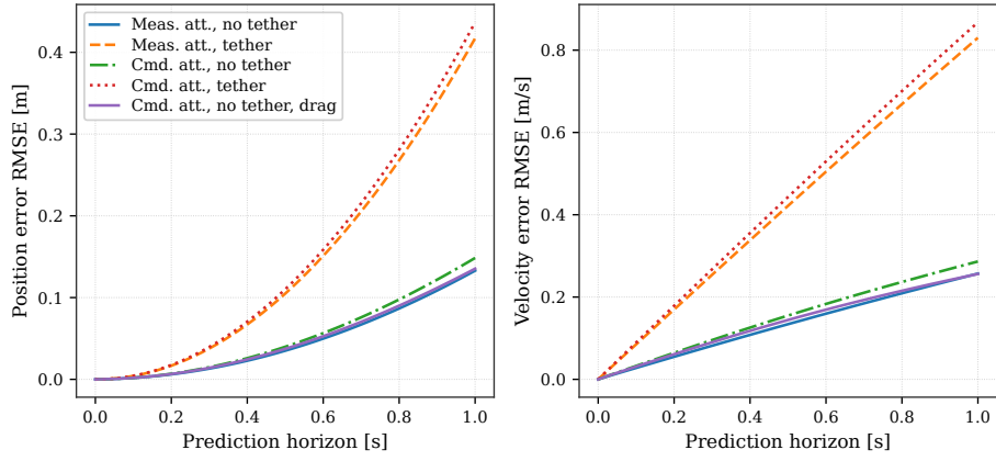
Figure 4.17: UAV prediction error as a function of the prediction horizon, for different model configurations.
